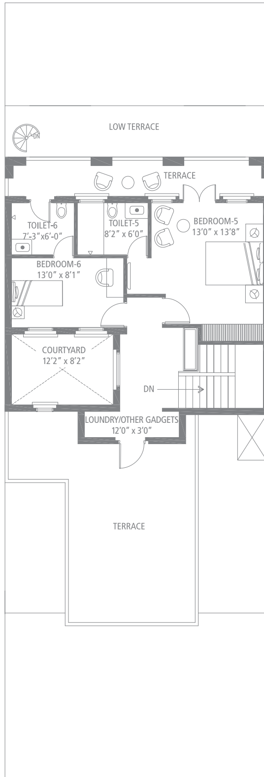
Second Floor
