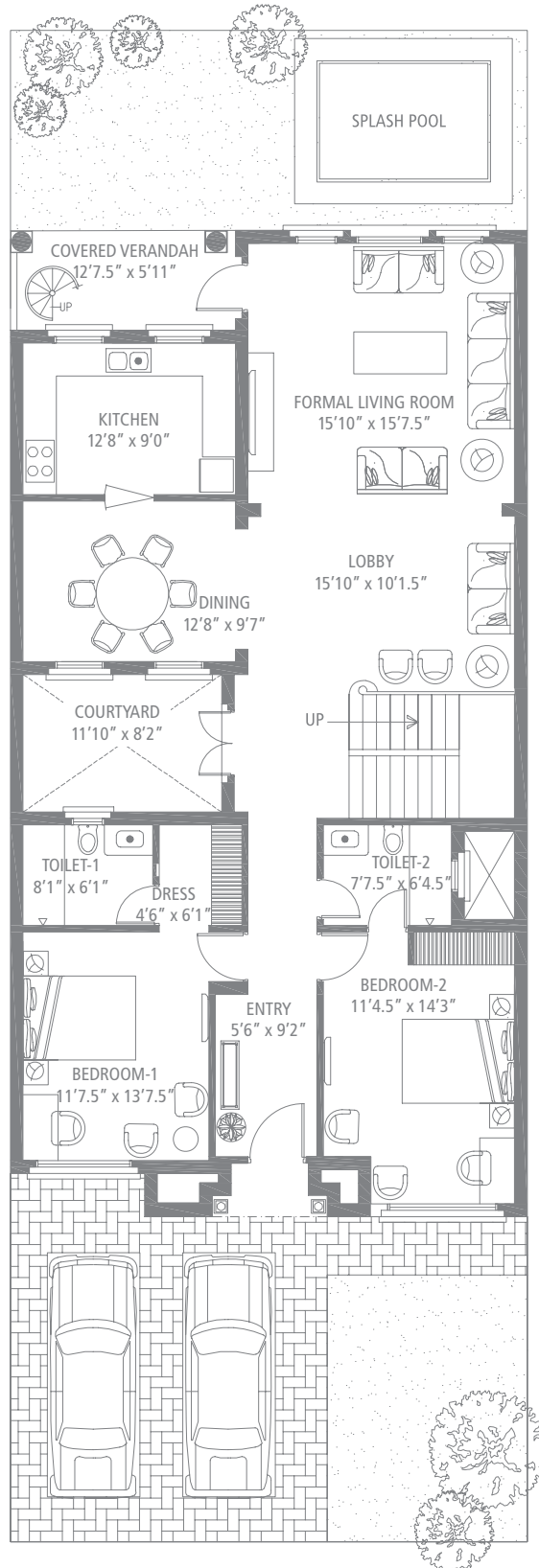
Ground Floor
